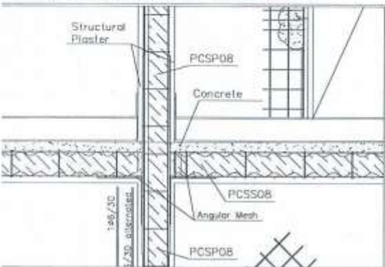
Figure 8. Building Details for Single Panel -- Sections
