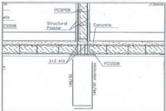
Figure 8. Building Details for Single Panel -- Sections
